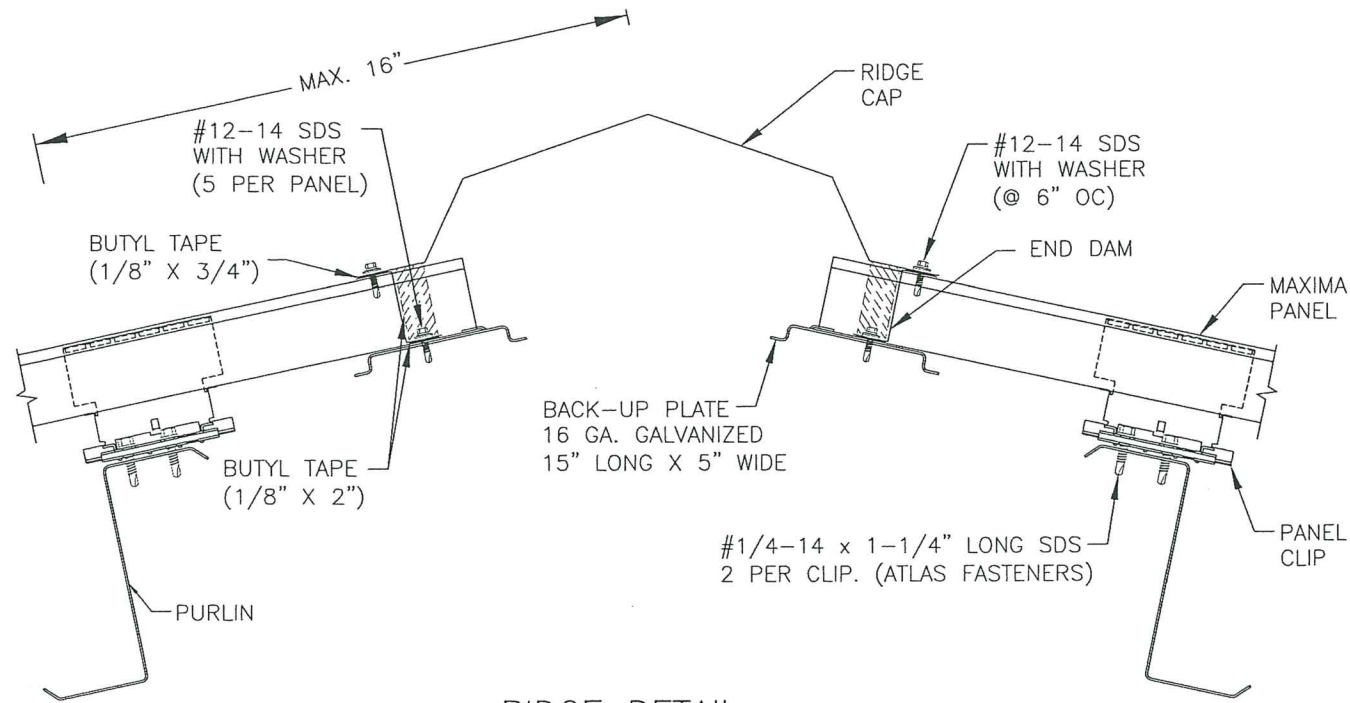
RIDGE DETAIL
