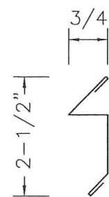
RAKE RETAINER TRIM (26 GA.)
