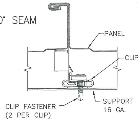
180° SEAM
