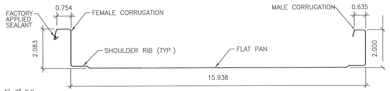
TYPICAL PANEL PROFILE 24 GA. GALVALUME COATED STEEL WITH PAINTED FINISH ( t = 0.0245 " MIN.)
