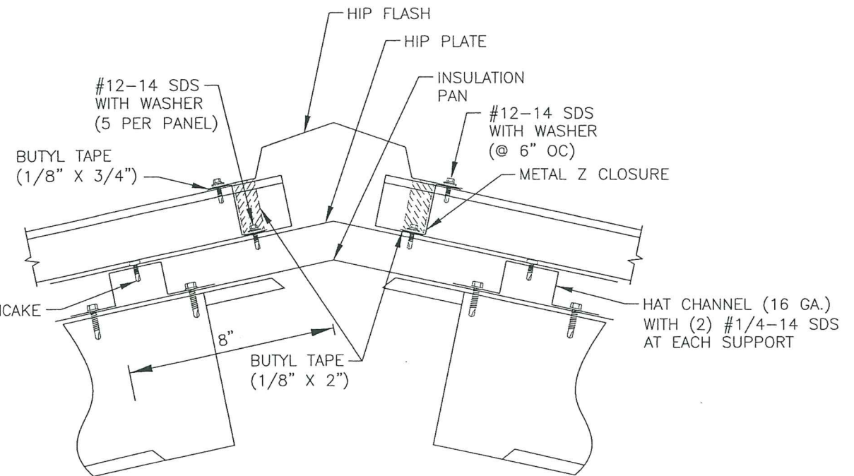
HIP DETAIL
