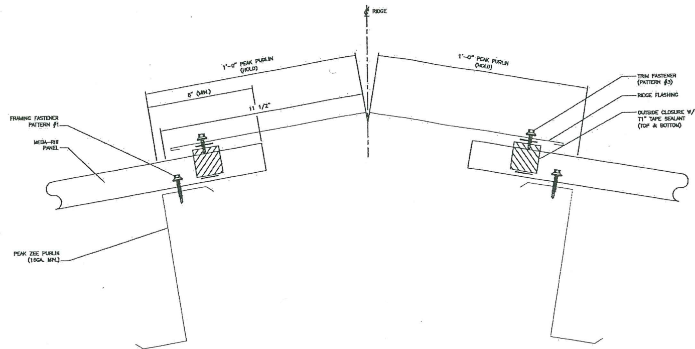
DETAIL © RIDGE
