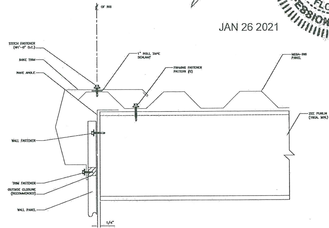
DETAIL © RAKE
