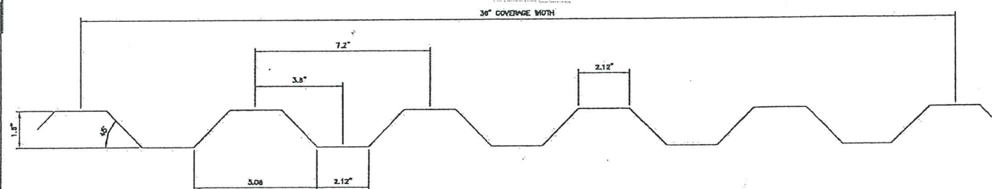
MEGA-RIB CROSS SECTION
