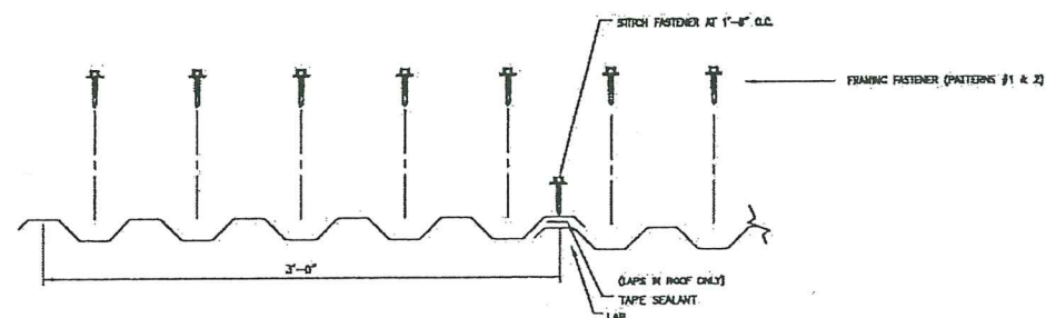
TYPICAL FRAMING AND STITCH FASTENER PATTERNS
