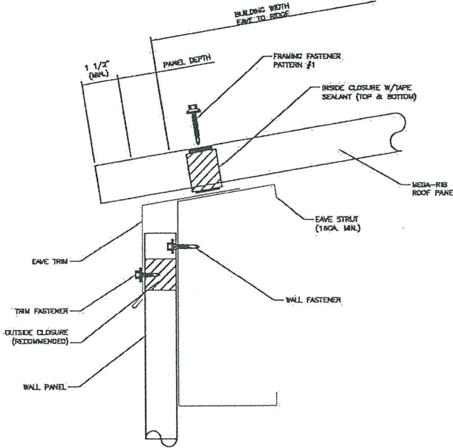
DETAIL @ EAVE
