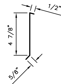
MT-156: RAKE SUPPORT CLEAT
