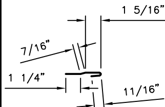
MT-11: VALLEY / WAVE CLIP
