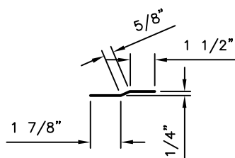
MT-38: STANDARD OFFSET CLEAT
