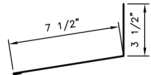
MT-35: STANDARD HEADWALL TRIM
