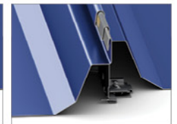
After Seaming
