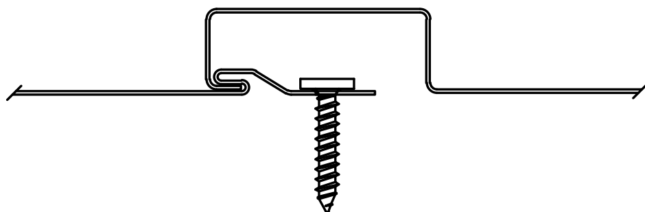
Typical Seam Engagement
