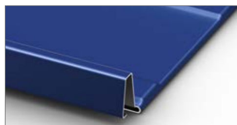
Eave Notch Folded in Field
