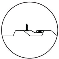
WAVE FLOATING SEAM ENGAGEMENT WAVE FLOATING UTILIZES SEPARATE CLIPS (SUBSTRATE & FOAM CLOSURES NOT SHOWN FOR CLARITY)
