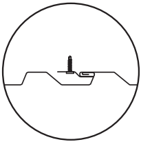
WAVE FIXED SEAM ENGAGEMENT
