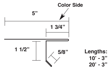
Arch Utility Offset Cleat MXUOF
