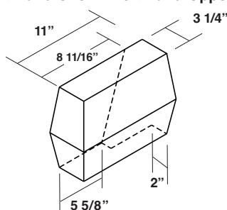
Gutter Corner Box for Standard Gutter 2:12 to 4:12 pitch or with Sculptured Gutter (Right Hand Shown-Left Hand Opposite)
