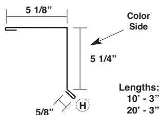
Arch Rake Trim MXART
