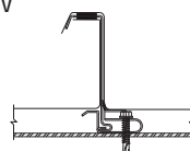
Maxima ADV Without Shoulders 180° Fold
