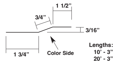
Arch Perimeter Cleat MXAPC
