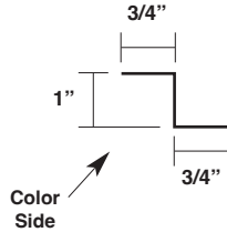
Gutter Strap ML-GS
