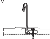
Maxima ADV Without Shoulders Before Mechanical Seaming
