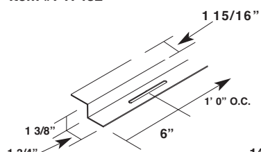
High Floating Rake Plate Item #: 17482
