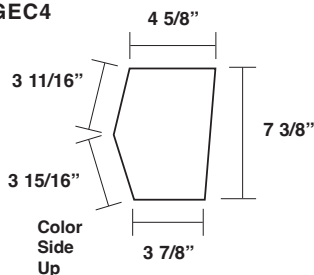
Gutter End Cap Over 2:12 TO 4:12 Pitch MX2GEC4
