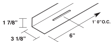
Maxima 3" Rake Support Angle Primed High Floating x 10' Item #: 17531
