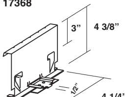
3:24 High Floating Clip Item #: 17368
