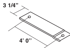
4' Back-Up Channel - Galvanized Item #: 17400
