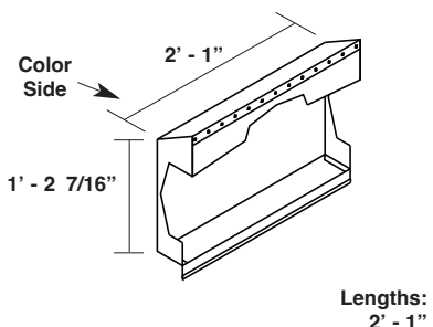
Gutter Corner Box for Sculptured Eave Up to 4:12 Pitch MLGCB
