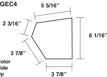
Gutter End Cap Over 2:12 TO 4:12 Pitch MLGEC4
