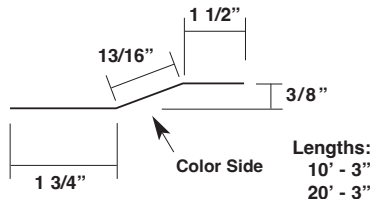
Arch Rake Tie-In Trim MXAEW
