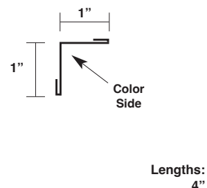
Outside Corner Box for Standard Gutter** Up to 2:12 Pitch MLOCB2
