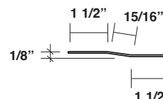
Utility Eave Plate Item #: 17477 Primed Item #: 221025 Galvanized
