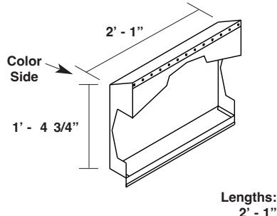
Hi-Side Corner Box MLHCB
