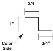
Gutter Strap ML-GS
