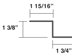
Standard Back-Up Plate Galvanized 16" Item #: 17330 18" Item #: 17332 24" Item #: 17334
