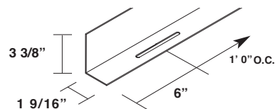
Maxima 2" / ADV Rake Support Angle Primed High Floating x 10' Item #: 17529
