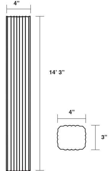
Downspout BBPDS
