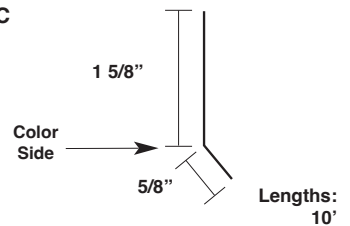
Arch Perimeter Cleat MXAPC
