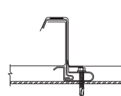
Maxima 1.5 Before Mechanical Seaming
