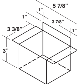
Lock-Seam Downspout Outlet - Standard
