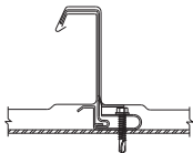
Maxima Before Mechanical Seaming
