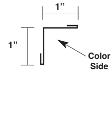
Outside Corner Box for Standard Gutter** Up to 2:12 Pitch MLOCB2
