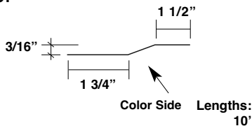
Zee Closure MDLZC
