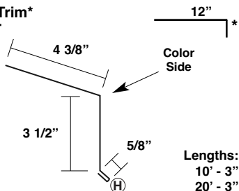
Perimeter Cleat MDPC
