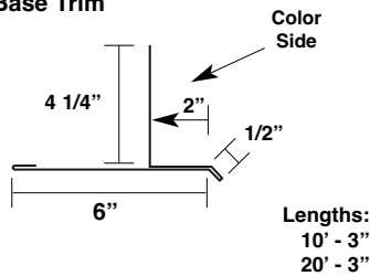
Outside Corner MDOC
