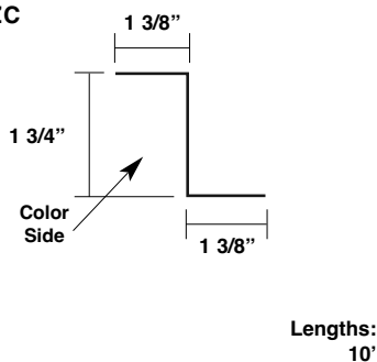
Hi-Side Tie-In Trim* MDSW
