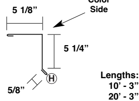
Vented Zee Closure
