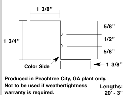
Hip Flashing* MDHF
