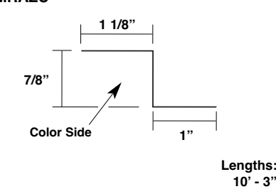
High Side Tie-In Trim* MRESW
