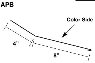
Pitch Break MRAPB
