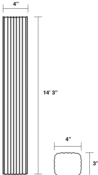
Downspout BBPDS
