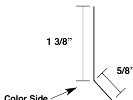
Perimeter Cleat MRAPC
