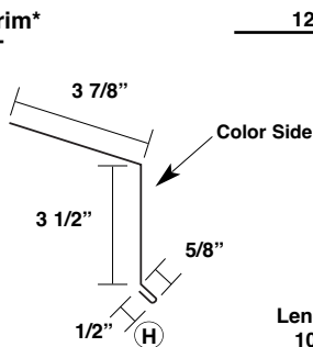
Eave Drip 1.5" MRAM15EDT
