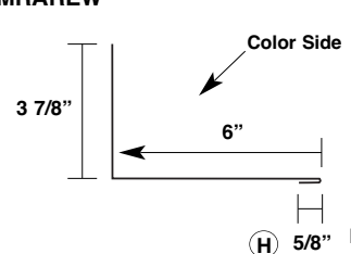
Sidewall Trim MRAREW
