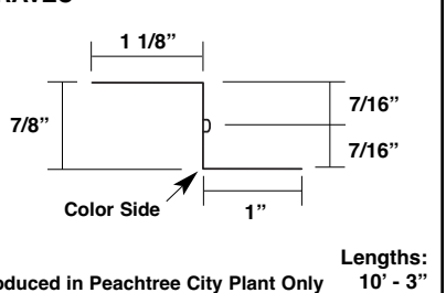
Hip Trim* MRHT
