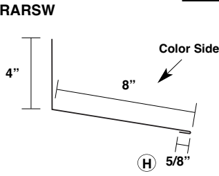
Endwall Trim MRARSW
