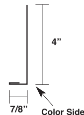
Angle Trim 7/8" x 4" MTA4
