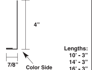
Angle Trim 7/8" x 4" MTA4
