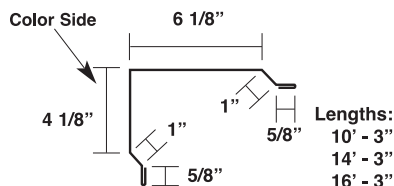
High Side Trim* P-HSE
