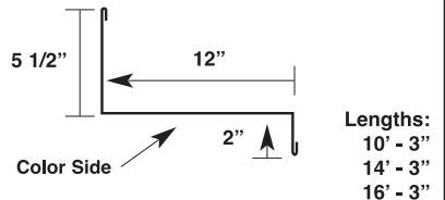
Eave FLASHING* (P-EF)*
