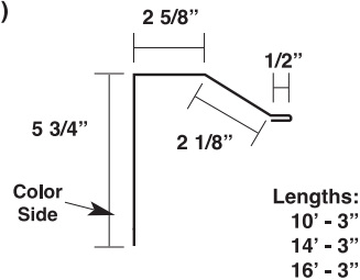
Door Track Cover (Cannonball Facemount) (P-DTC-CB)
