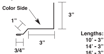
Rake Tie-In Trim (P-EWF)
