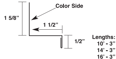
Square Base (P-SQB)
