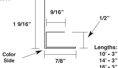
Matrix F x 1/2" MTF
