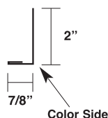
Angle Trim 7/8" x 2" MTA2
