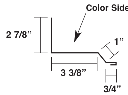
Rake Tie-In (R-EW)
