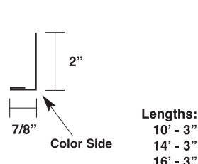
Angle Trim 7/8" x 2" MTA2
