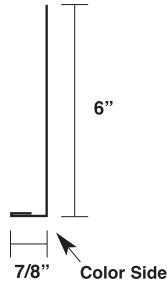
Angle trim - 7/8 x 6" MTA6
