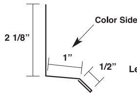
Base Drip P-DF
