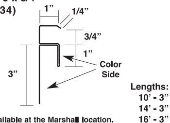
F and J x 3/4" (P-FJ34)
