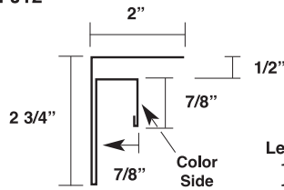
Matrix F and J x 1/2" MTFJ12
