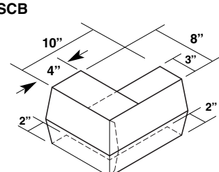
High Side Corner Box (Right Hand Shown Left Hand Opposite) ITHSCB
