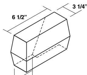
Gutter Corner Box For Sculptured Gutter (Right Hand Shown Left Hand Opposite) ITGCB
