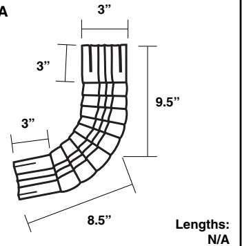
Lock-Seam Downspout Outlet - Standard
