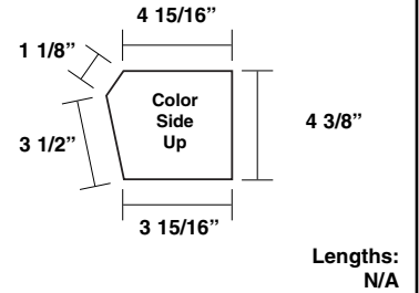
Aluminum Downspout Outlet Box BBPOUT
