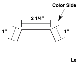
Downspout Strap BBPDSS
