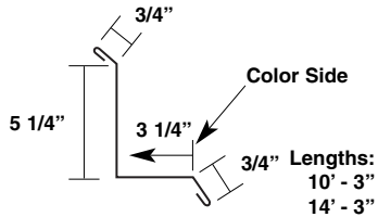
Inside Corner MGIC
