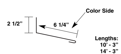
Variable Peak Box IT-PBV
