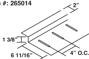
High Floating Eave Plate Item #: 265014
