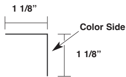
Insulation Angle Trim MLIA
