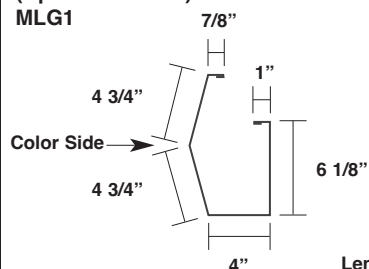
Gutter (Up to 2:12 Pitch) MLG1
