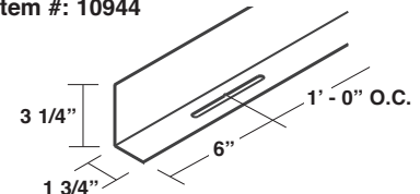
Low Floating Rake Support Angle Item #: 10944
