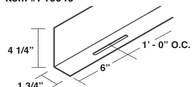
High Floating Rake Support Angle Item #: 10946
