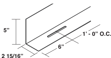
MLFS Tall Floating Rake Support Angle Item #: 232319
