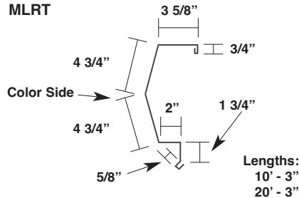
Rake Tie-In Trim
