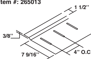
Low Floating Eave Plate Item #: 265013
