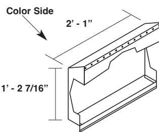
Floating Peak Box (Up to 2:12 Pitch) MLFLPB1
