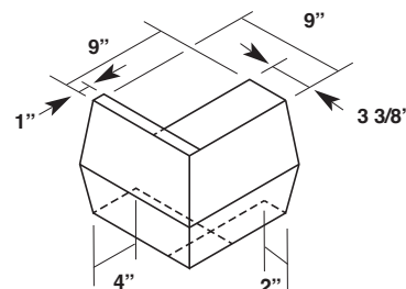
Outside Corner Box for Standard Gutter Up to 2:12 Pitch
