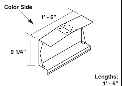
Fixed Peak Box (Up to 2:12 Pitch) MLFXPB1
