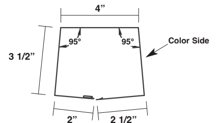
Lock-Seam Downspout - Center
