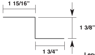
High Eave Plate Item #: Galvanized: 211274 Red Primed: 237215
