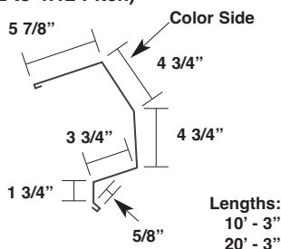
Fixed Ridge Flashing* (Up to 4:12 Pitch) MFXR1
