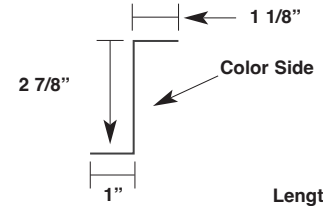
Aluminum Downspout Outlet Box BBPOUT
