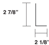
Utility Fixed Rake Support Angle Item #: 10' - 11213 Item #: 20' - 11196
