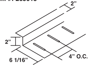
MLFS Tall Floating Eave Plate Item #: 265015
