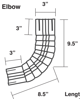
Lock-Seam Downspout - Center
