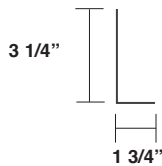
Low Fixed Rake Support Angle Item #: 10' - 11005 Item #: 20' - 10941
