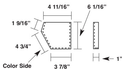
Gutter End Cap (Up to 2:12 Pitch) MLGE1
