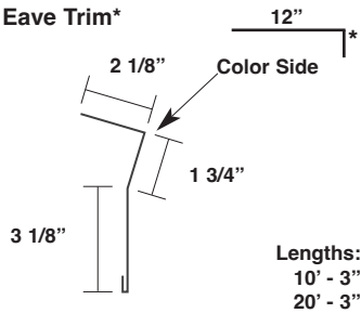
Sculptured Eave Trim* MLSCE
