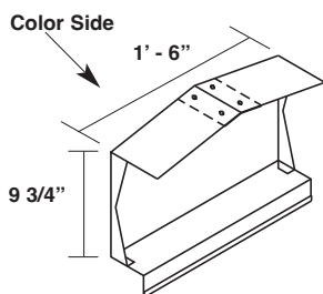
Fixed Peak Box (Over 2:12 to 4:12 Pitch) MLFXPB4
