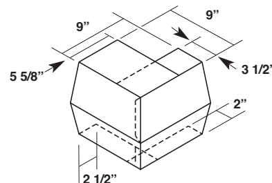
High Eave Corner Box (Right Hand Shown-Left Hand Opposite)
