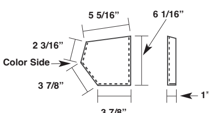
Gutter End Cap (Over 2:12 to 4:12 Pitch) MLGE4
