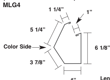
Gutter (Over 2:12 to 4:12 Pitch) MLG4
