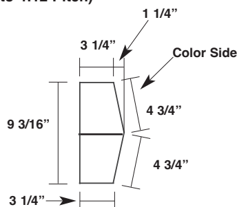
Gutter Corner Box for Sculptured Eave (Up to 4:12 Pitch)
