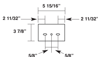
Bearing Plate Primed Item #: 94599 Galvanized Item #: 203541
