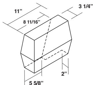
Outside Corner Box for Standard Gutter 2:12 to 4:12 pitch
