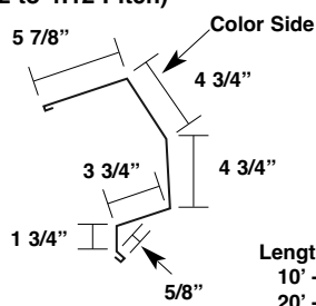
Fixed Ridge Flashing* (Up to 4:12 Pitch) MFXR1
