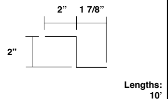
Bearing Plate Primed Item #: 94599 Galvanized Item #: 203541
