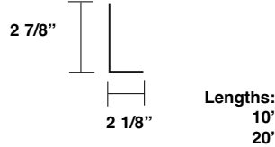
Utility Floating Rake Support Angle Item #: 10942
