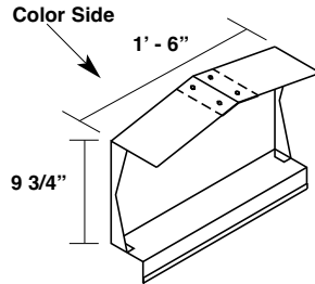
Fixed Peak Box (Over 2:12 to 4:12 Pitch) MLFXPB4
