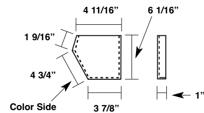
Gutter End Cap (Up to 2:12 Pitch) MLGE1
