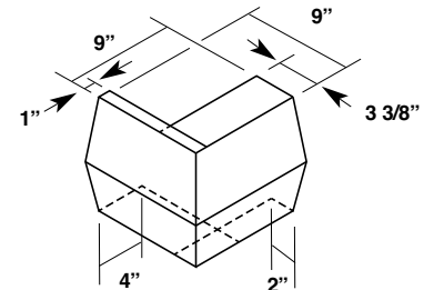
Outside Corner Box for Standard Gutter Up to 2:12 Pitch
