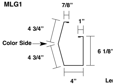
Gutter (Up to 2:12 Pitch) MLG1
