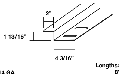
Standard Back-Up Plate for 24" Wide Panels Item #: 10949
