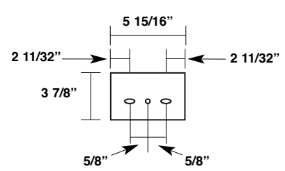
Standard Back-Up Plate for 18" Wide Panels Item #: 10950
