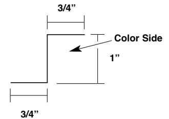
Gutter Strap ML-GS
