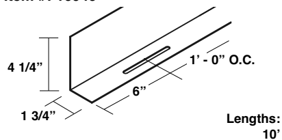
MLFS Tall Floating Rake Plate Item #: 232318
