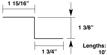
High Fixed Rake Support Angle Item #: 10' - 11002 Item #: 20' - 10943
