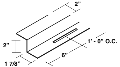
MLFS Tall Floating Rake Plate Item #: 232318
