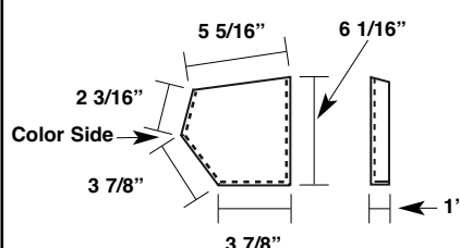
Gutter End Cap (Over 2:12 to 4:12 Pitch) MLGE4
