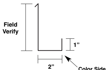
Zee Closure MT-184
