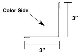
**Inside Corner Trim MT-198
