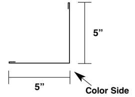
**Outside Corner Trim MT-197
