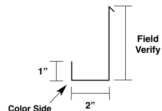
Jamb Trim - Notched (Left) (Houston Plant Only) MT-173L
