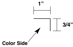
**Inside Corner Trim MT-198
