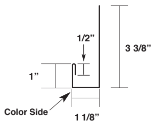
"J" Trim MT-49
