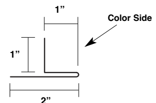
Outside Corner Cleat - Notched (Right) (Houston Plant Only) MT-175
