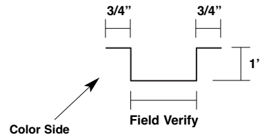
Reveal Closure MT-195
