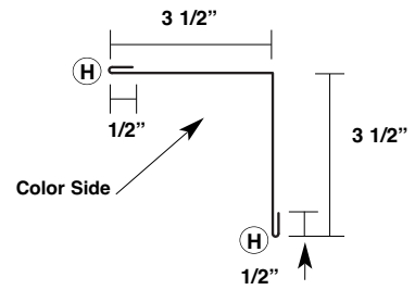
Inside Corner Trim MT-56
