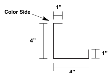
Outside Corner Trim - Notched MT-WAV-CRN-OS-STD
