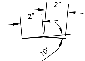
BEND PLATE (FOR UP TO 2:12 PITCH)
