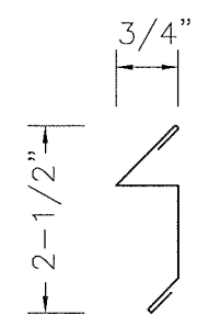
RAKE RETAINER TRIM (26 GA.)
