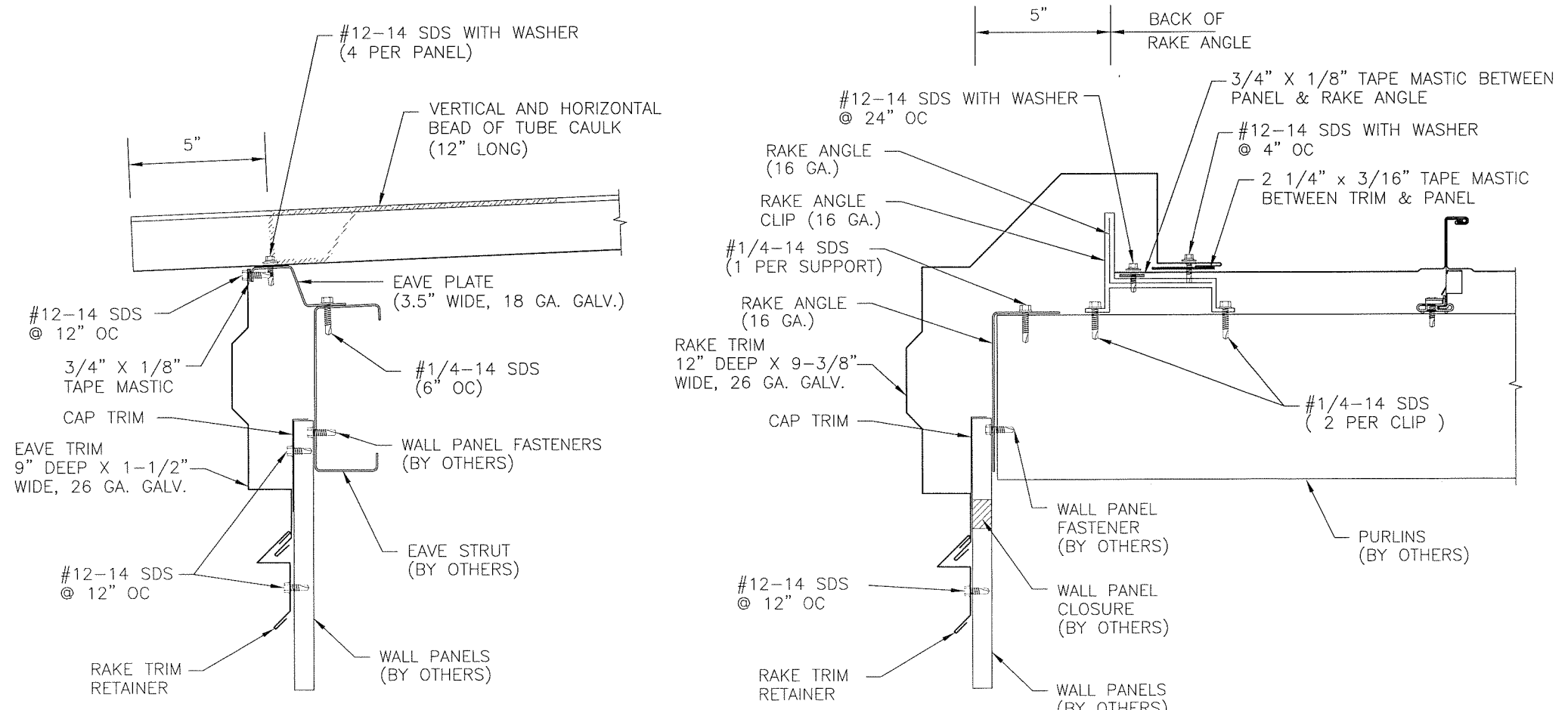
SECTION EAVE DETAIL (C/2)
