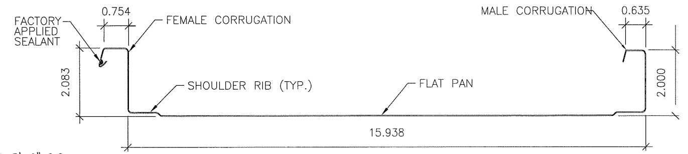
24 GA. GALVALUME COATED STEEL WITH PAINTED FINISH ( t = 0.0245 " MIN.)
