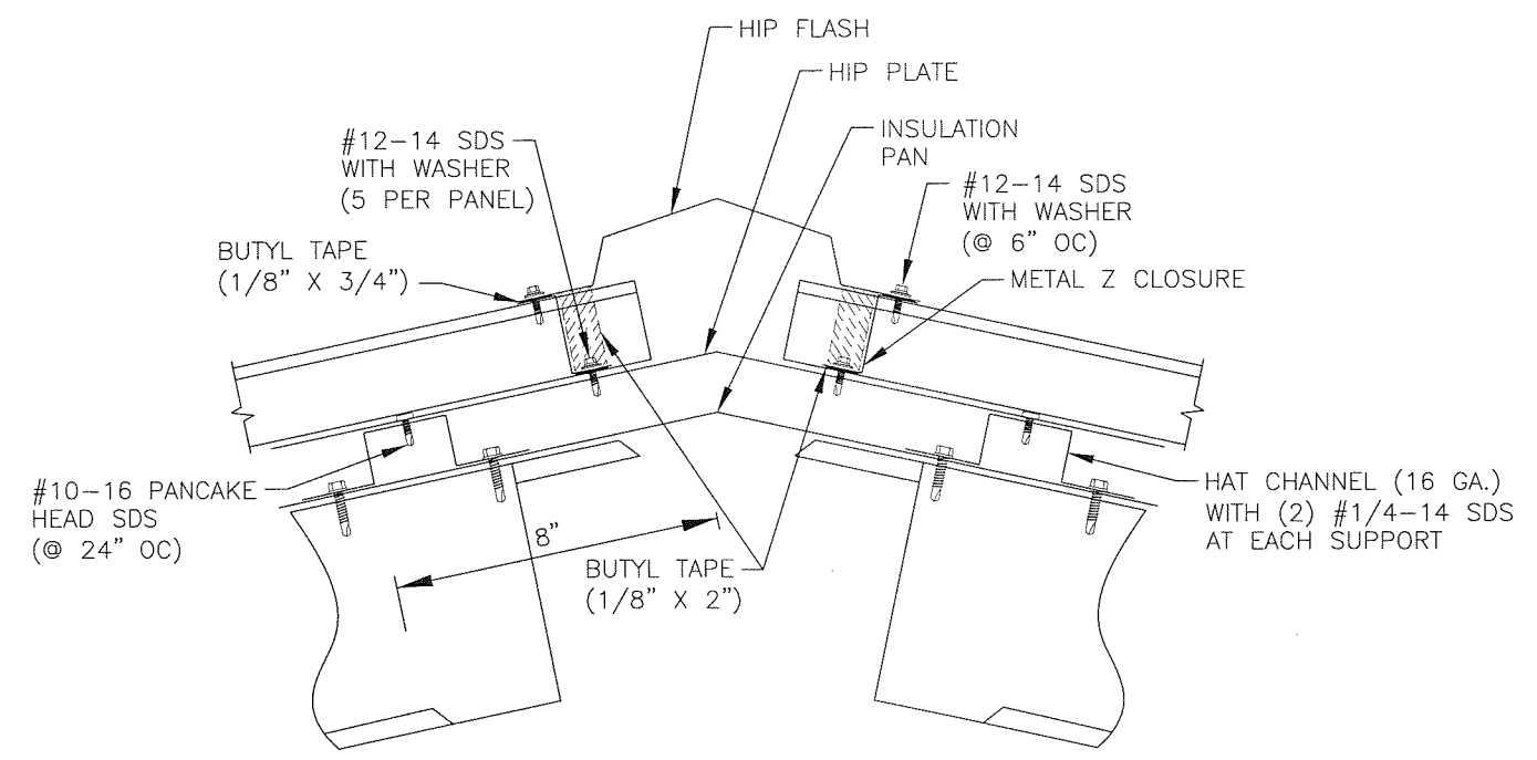
HIP DETAIL
