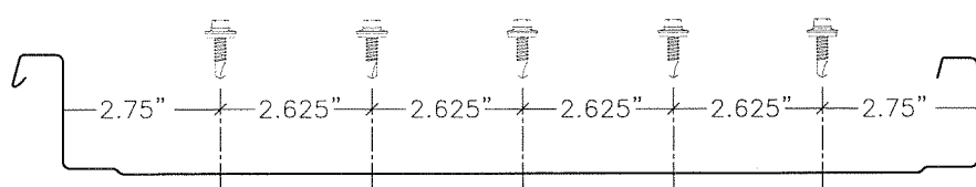
FASTENER PATTERN AT ENLAP
