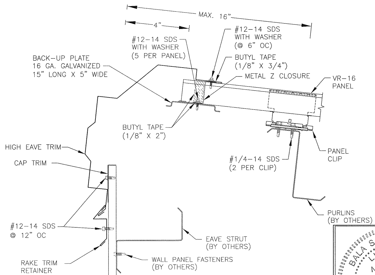
HIP DETAIL
