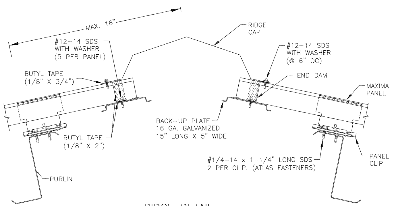
RIDGE DETAIL
