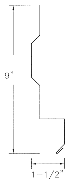
EAVE TRIM (26 GA.)
