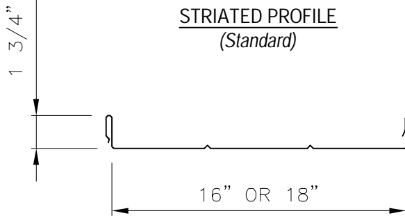
BEAD (PENCIL RIB) PROFILE (Optional)
