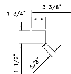
EAVE DRIP/RAKE TRIM
