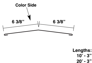
Hip Flashing* MDHF
