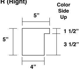
Gutter End Cap MDGECL (Left) MDGECR (Right)
