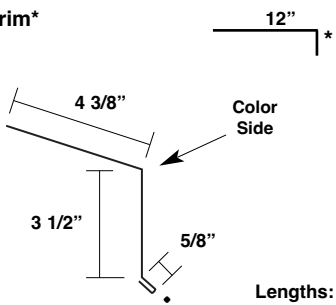
Perimeter Cleat MDPC
