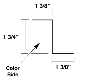
Zee Closure MDLZC
