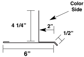
Soffit Base Trim MDSB
