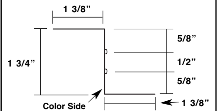
Vented Zee Closure
