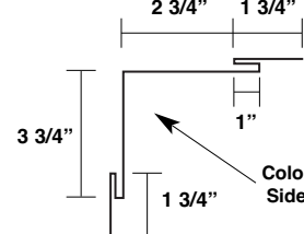
Inside Corner MDIC
