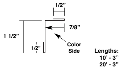
Zee Closure MDLZC
