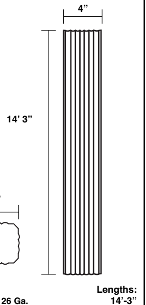
Downspout BBPDS
