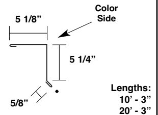
Vented Zee Closure
