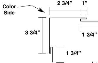
Outside Corner MDOC
