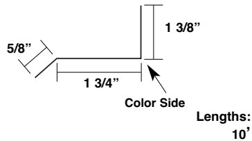
Angle Trim MDAN
