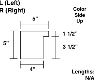
Downspout Strap BBPDSS
