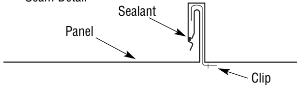
Medallion-Lok Seam Detail
