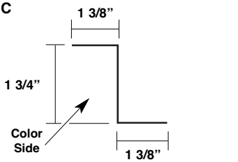
Zee Closure MDLZC
