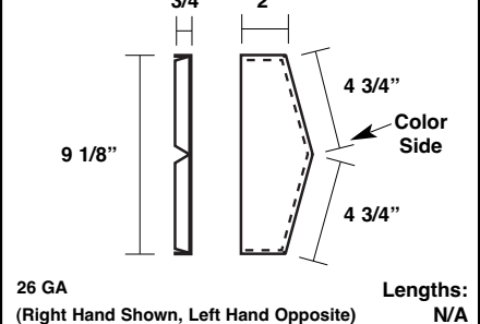
High Side Eave Trim (Up to 2:12 Pitch) MLHS2
