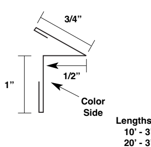
Alternate Rake Tie-In Trim
