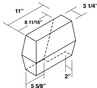
Outside Corner Box for Standard Gutter 2:12 to 4:12 pitch or with Sculptured Gutter MLOCB4
