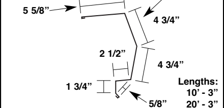
Floating High Side Tie-In* MLFLHST
