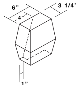
Gutter Corner Box for Sculptured Eave (Up to 4:12 Pitch) MLGCB
