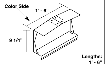
Fixed Peak Box (Up to 2:12 Pitch) MLFXPB2
