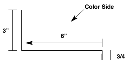
Alternate Rake Tie-In Trim
