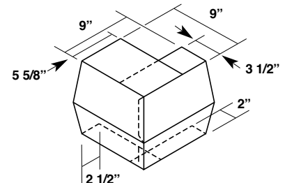
High Side Corner Box MLHCB
