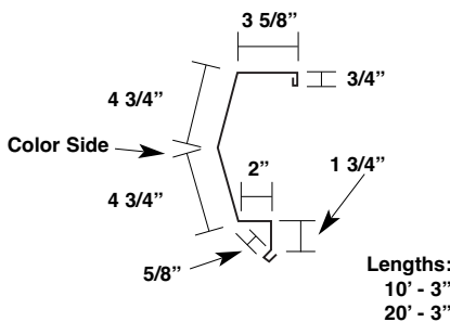
Rake Tie-In Trim
