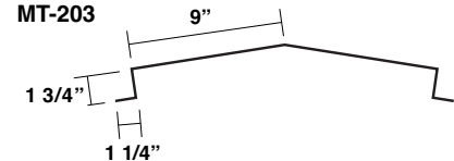
1 3/4" Offset Hip/Ridge Plate MT-203
