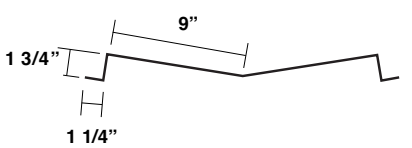
1 3/4" Offset Valley Plate MT-201
