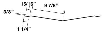
1 3/4" Offset Hip/Ridge Plate MT-203
