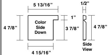
Gutter End Cap for Standard Box Gutter & Flanged Box Gutter MT-68R = Right End Cap MT-68L = Left End Cap
