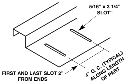
High Floating Eave Plate MT-208
