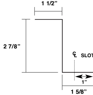
Slotted Starter Zee MT-SLOT-Z238
