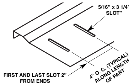
Low Floating Eave Plate MT-209
