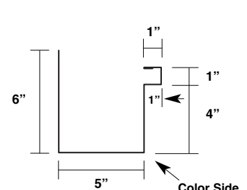
Standard Box Gutter MT-61
