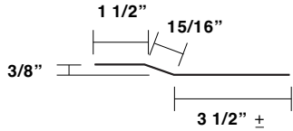
Low Eave Plate MT-185
