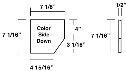
Gutter End Cap for 7" Box Gutter MT-69R = Right End Cap MT-69L = Left End Cap
