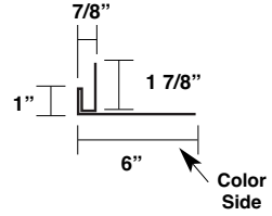
Overhead Door Flashing 8 7/8" (P-JF-B-8 7/8)
