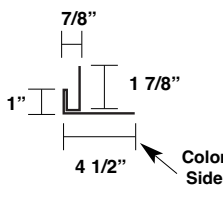
Overhead Door Flashing 8" (P-JF-B-8)
