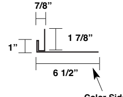
Walk Door (P-DWT) and Window Trim
