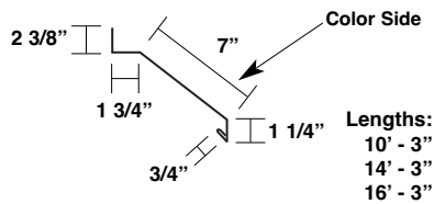
Soffit Flashing x 3 (P-SF3)
