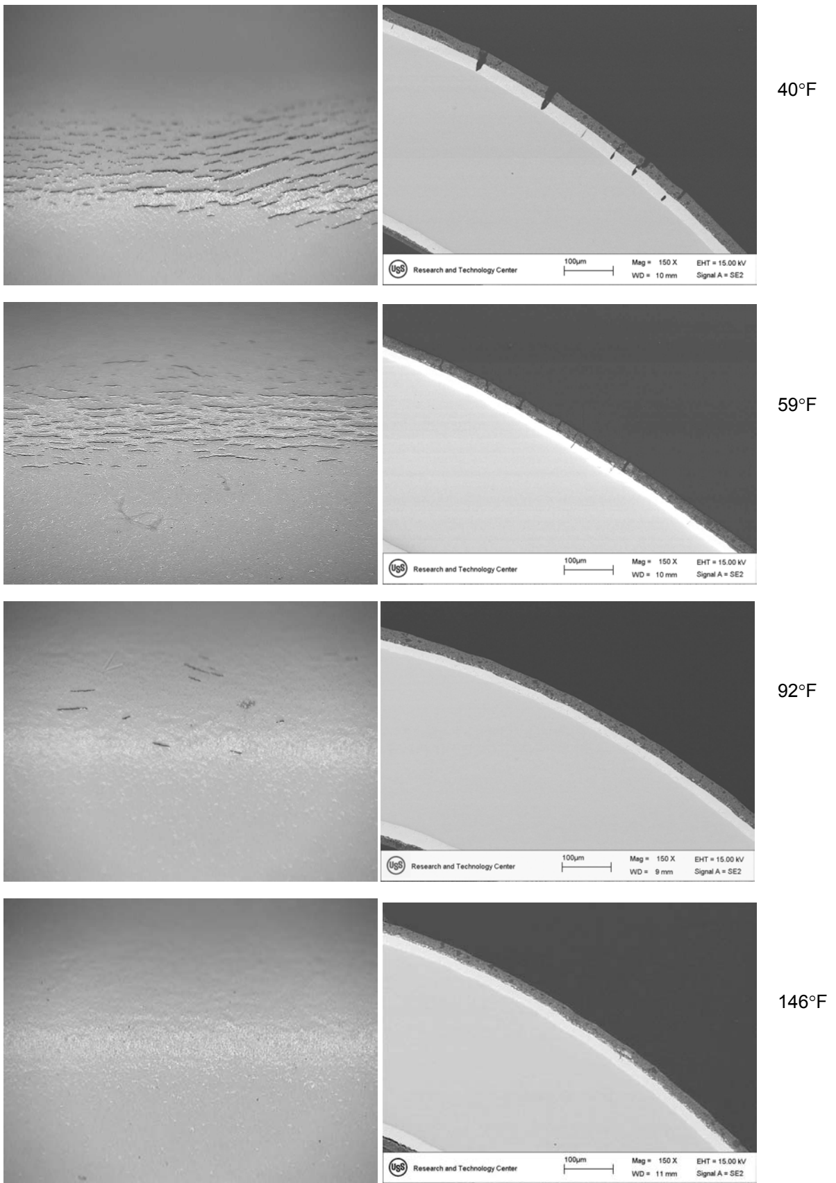
Figure 2. Optical micrographs of the surfaces and SEM micrographs of the cross-sections of prepainted HDG G100 at 30X and 150X magnifications, respectively. The panels were formed at different ambient temperatures, 40°F, 59°F and 92°F, with the heater off, and warm roll-formed at 146°F.
